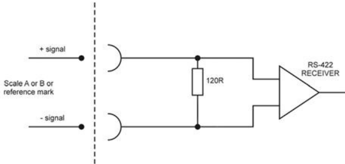
UCC T3 input circuits for CMM readhead - scale and reference mark inputs
